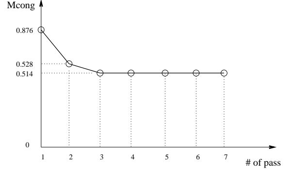
Figure 8: The convergence of maximum congestion in IFB phase for circuit apte.
