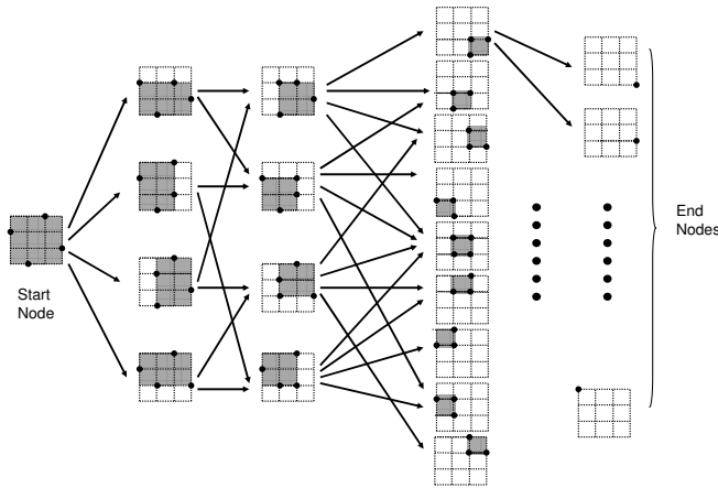
Fig. 5. Configuration Graph.
