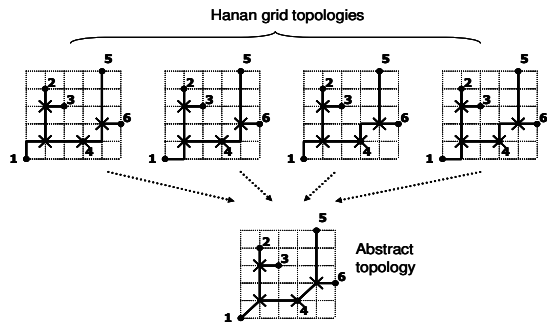
Fig. 6. Abstract topology.
