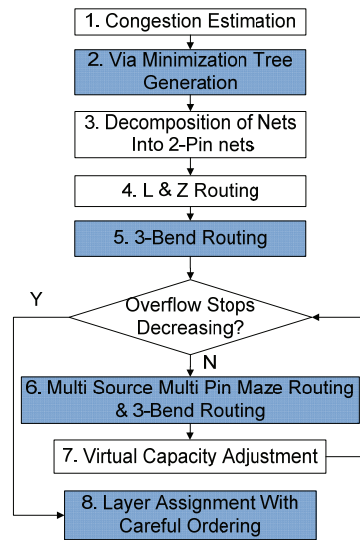
Fig. 2. FastRoute 4.0 Framework
