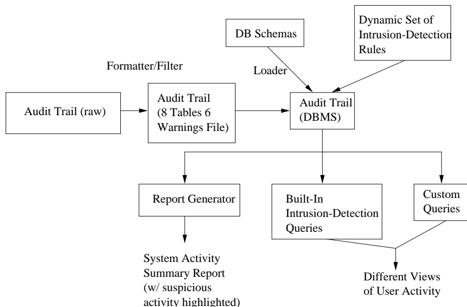
Figure 2.1: Dataflow diagram of ComputerWatch components (from [11])
